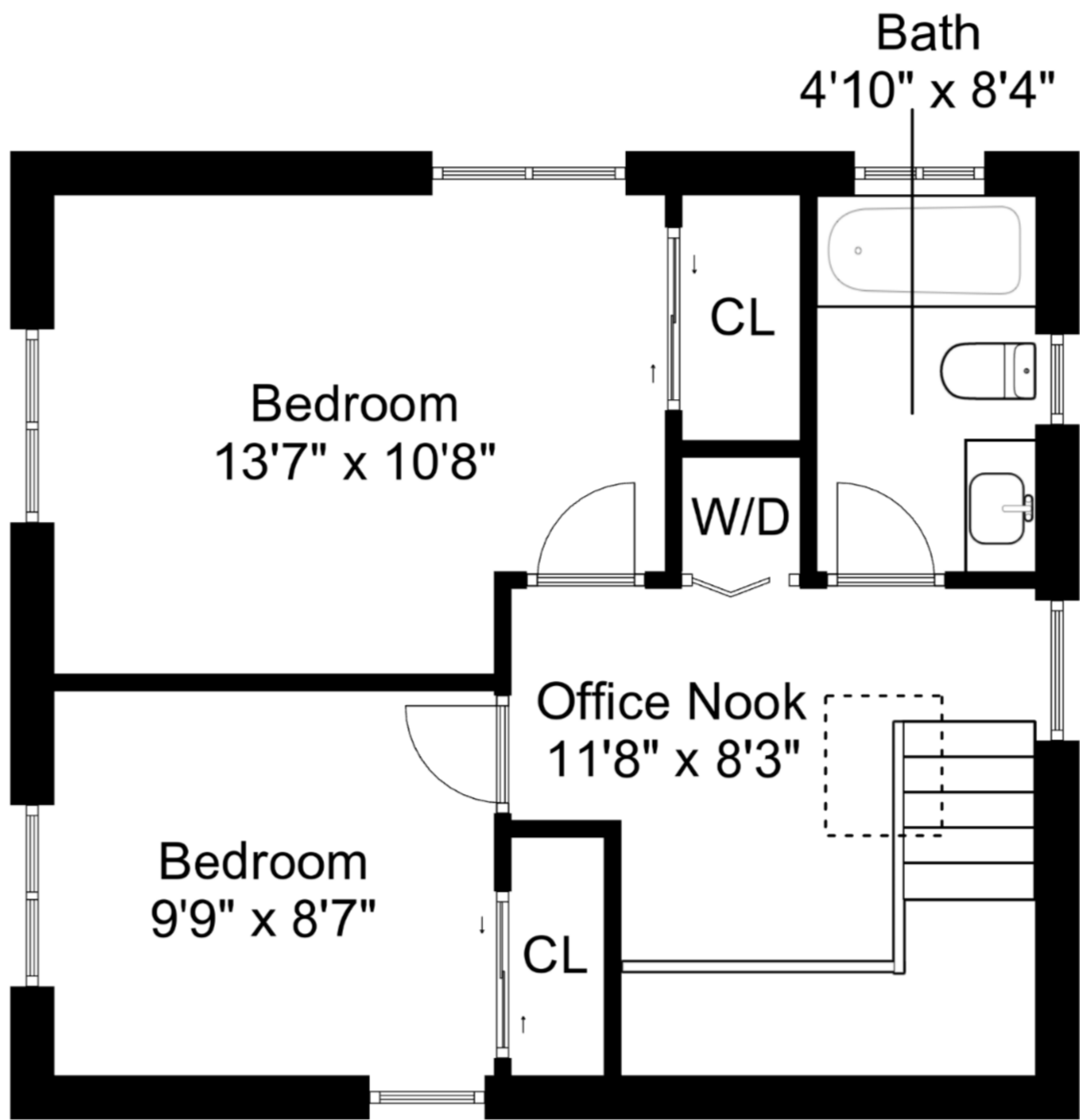
Upper Level
